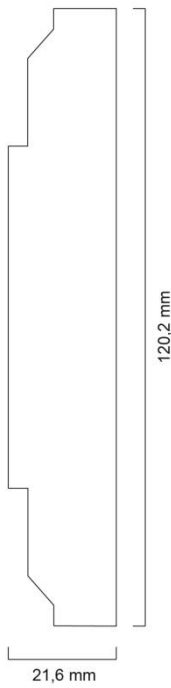
dimensions DALI Expander
