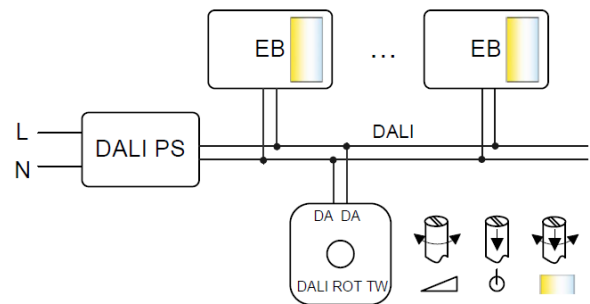
Application: tuneable white control using DALI ROT TW
