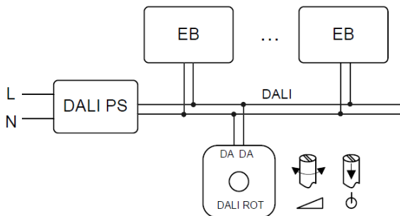
Application: switch and dim with DALI ROT module
