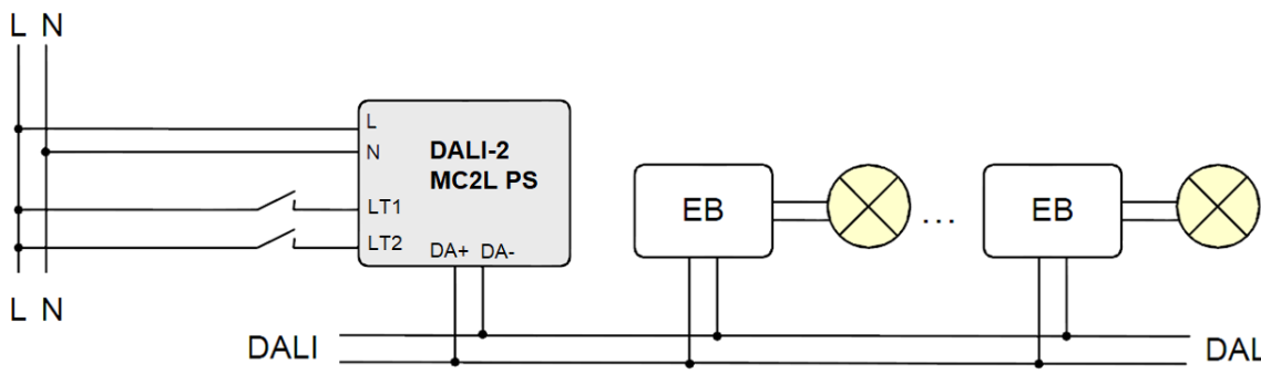
1 Typical Application, wiring diagram
