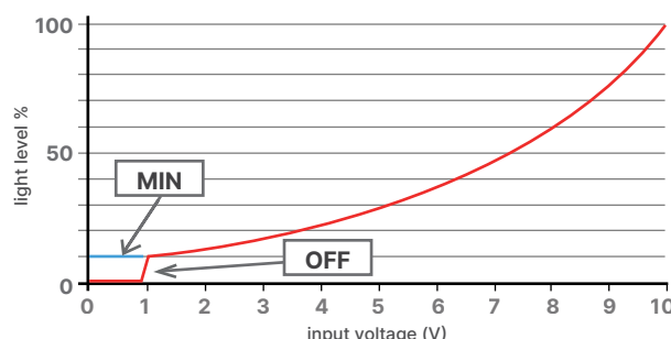
V4: Dimming: 10-100% <1V: MIN (10%) (blue curve)
